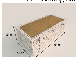
Earth lime platforms from water and food storage to raised farming.
