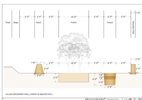
Village flood protection elements.
