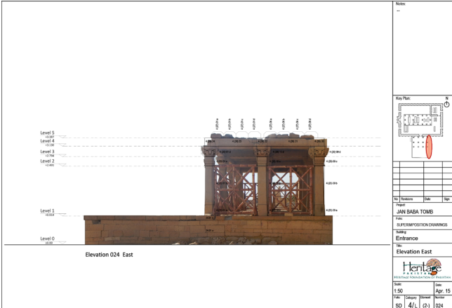
Photographic superimposition drawings for the Tomb of Jan Baba, WHS Makli.
